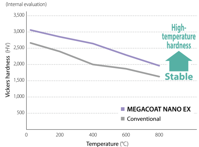
Comparison of vickers hardness transition with temperature (Internal evaluation)
